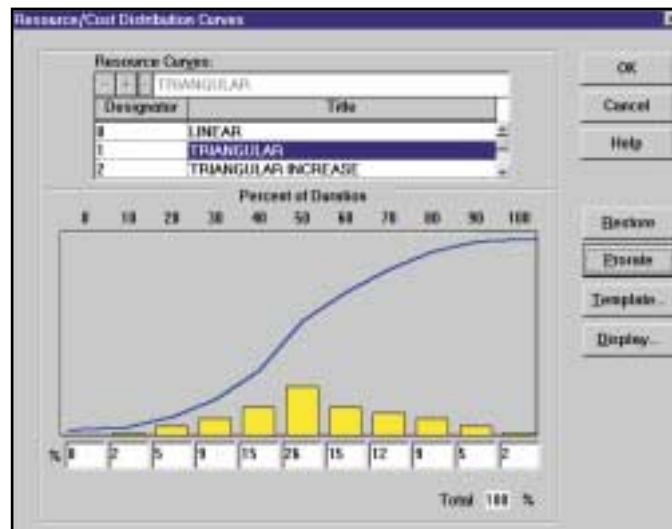
Use resource distribution curves to model how resources will be consumed as an activity progresses. Select from the library of predefined curves or quickly create your own.
